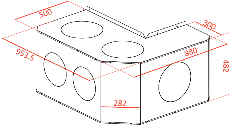
Article# 6004-Intake duct kit CT3500
