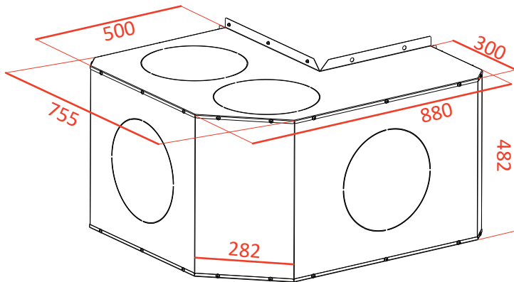
Article# 6005-Intake duct kit CT1000/CT2000
