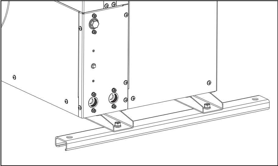
The hanging brackets are optional supplied for ceiling mounting
